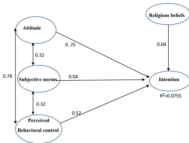
Figure 1. Structural Equation Model of Planned Behavior on Organ Donation Intention. Note. RMSAE: Root mean square error of approximation; \chi^2/df : Relative chi-square; DF: Degree of freedom; CFI: Confirmatory factor analysis; GFI: Goodness of fit index; TLI: Tucker-Lewis Index; NFI: Normed fit index; AGFI: Adjusted goodness of fit index. Chi-square: 1366.720, DF: 480; RMSAE: 0.053; \chi^2/df : 2.84; CFI: 0.916; GFI: 0.902; TLI: 0.908; NFI=0.877; AGFI: 0.878.
